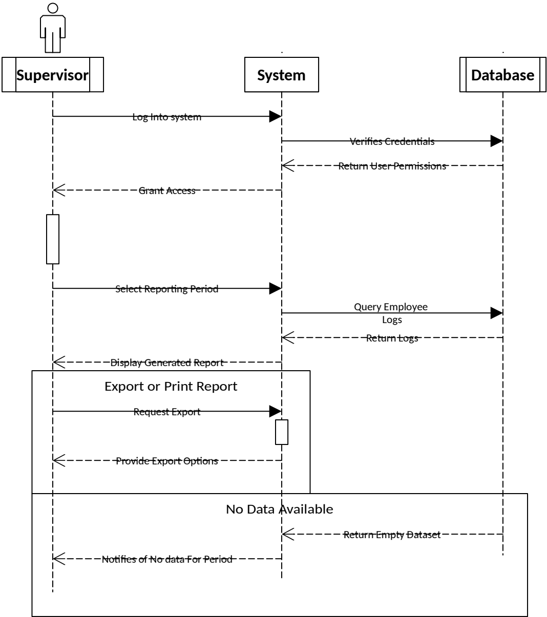
sequence diagram for the process
