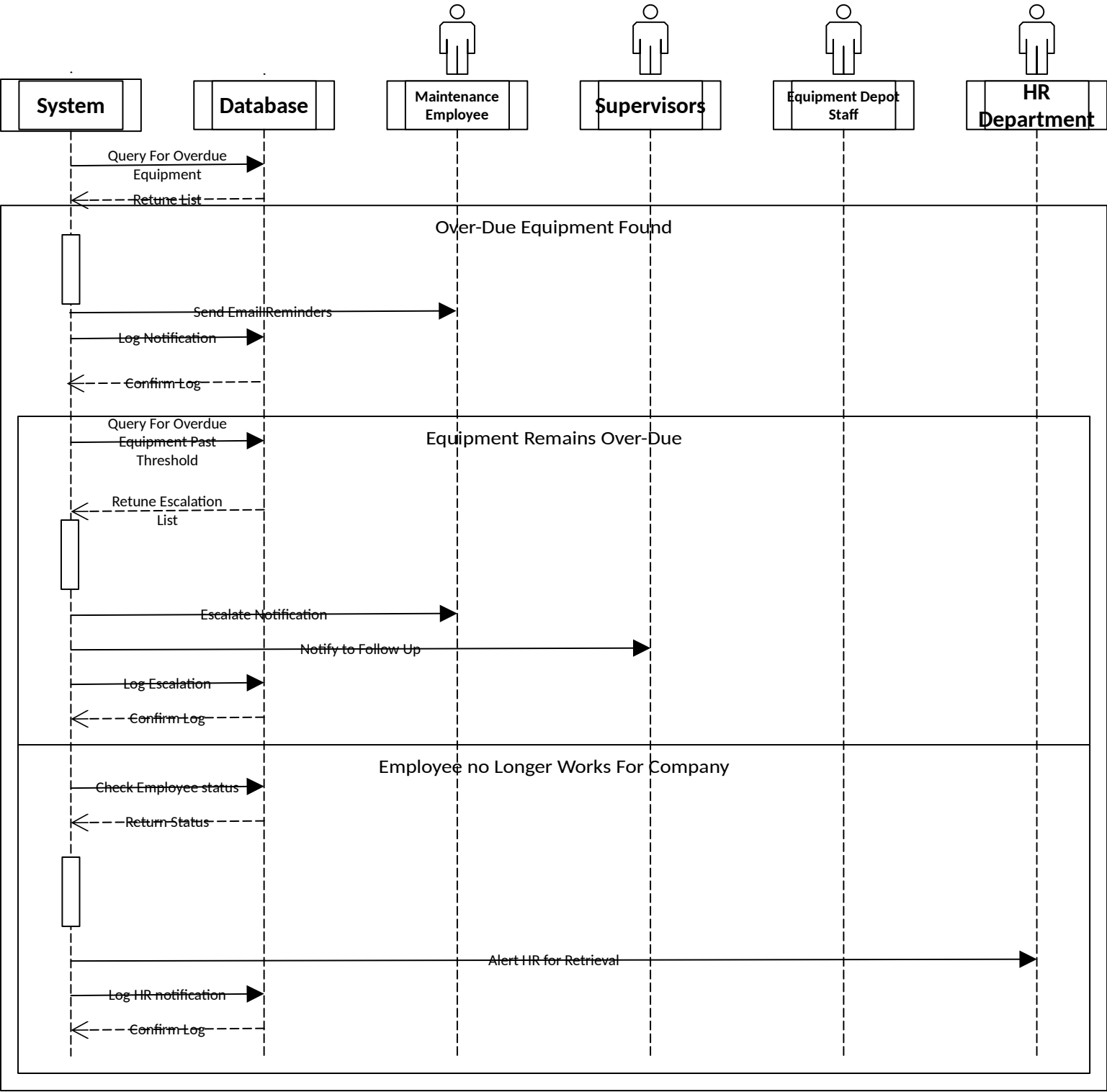
Sequence Diagram for Overdue Equipment Notification Process
