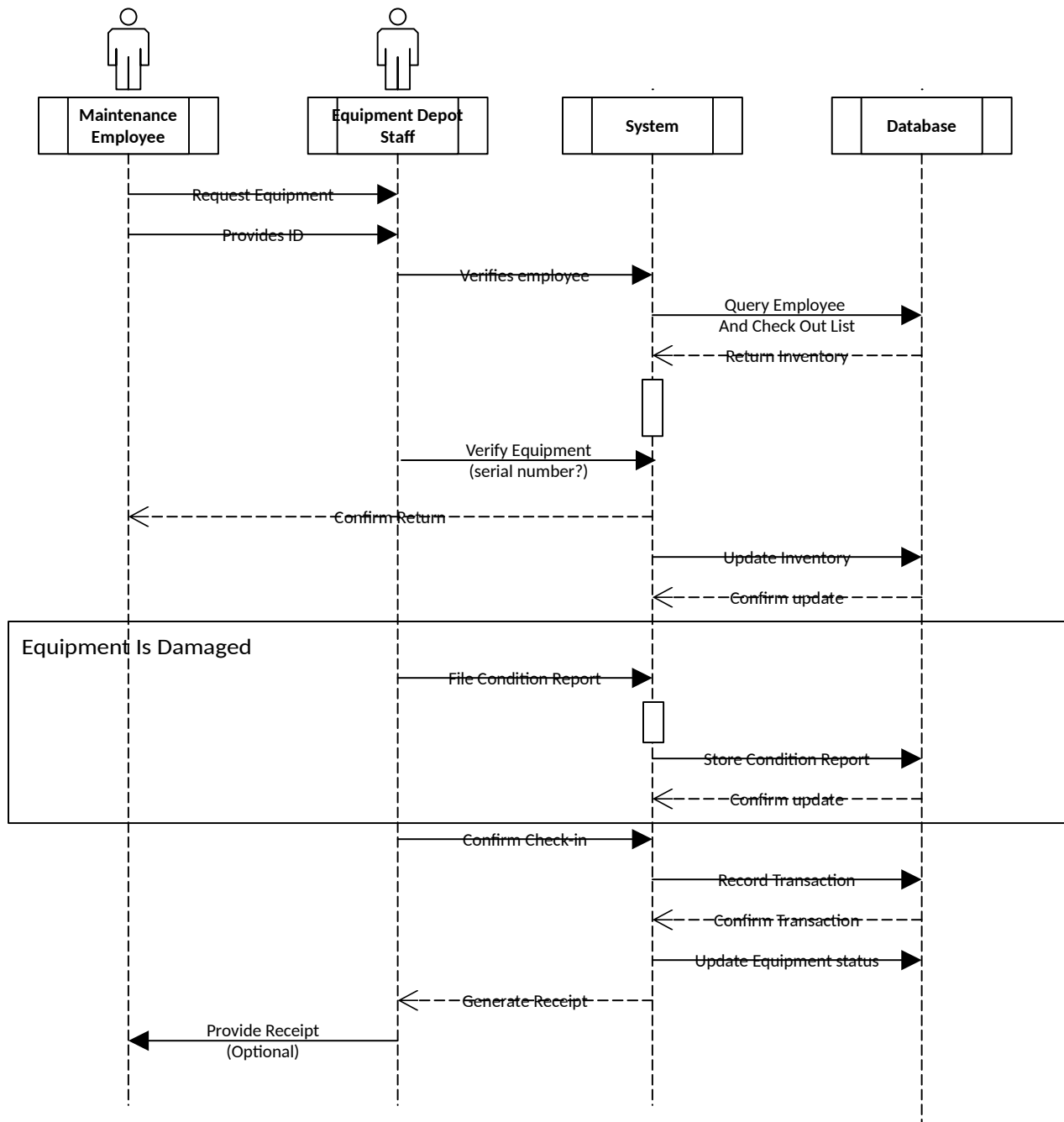
Sequence Diagram For The Check-in Process
